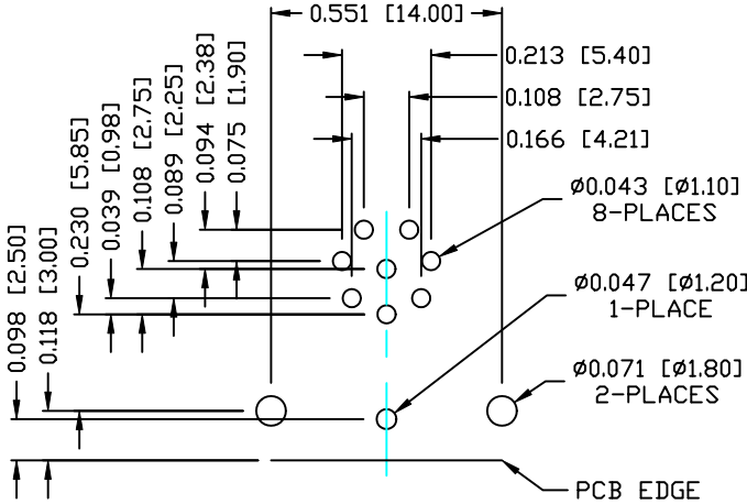
PCB LAYOUT
