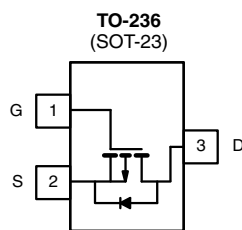
Top View SQ2309ES*
