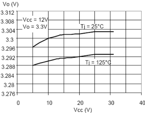
Figure 27. Line regulation
