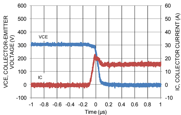
Figure 16. Turn-on waveform T_J=100^\circ C , V_{CC}=300V
