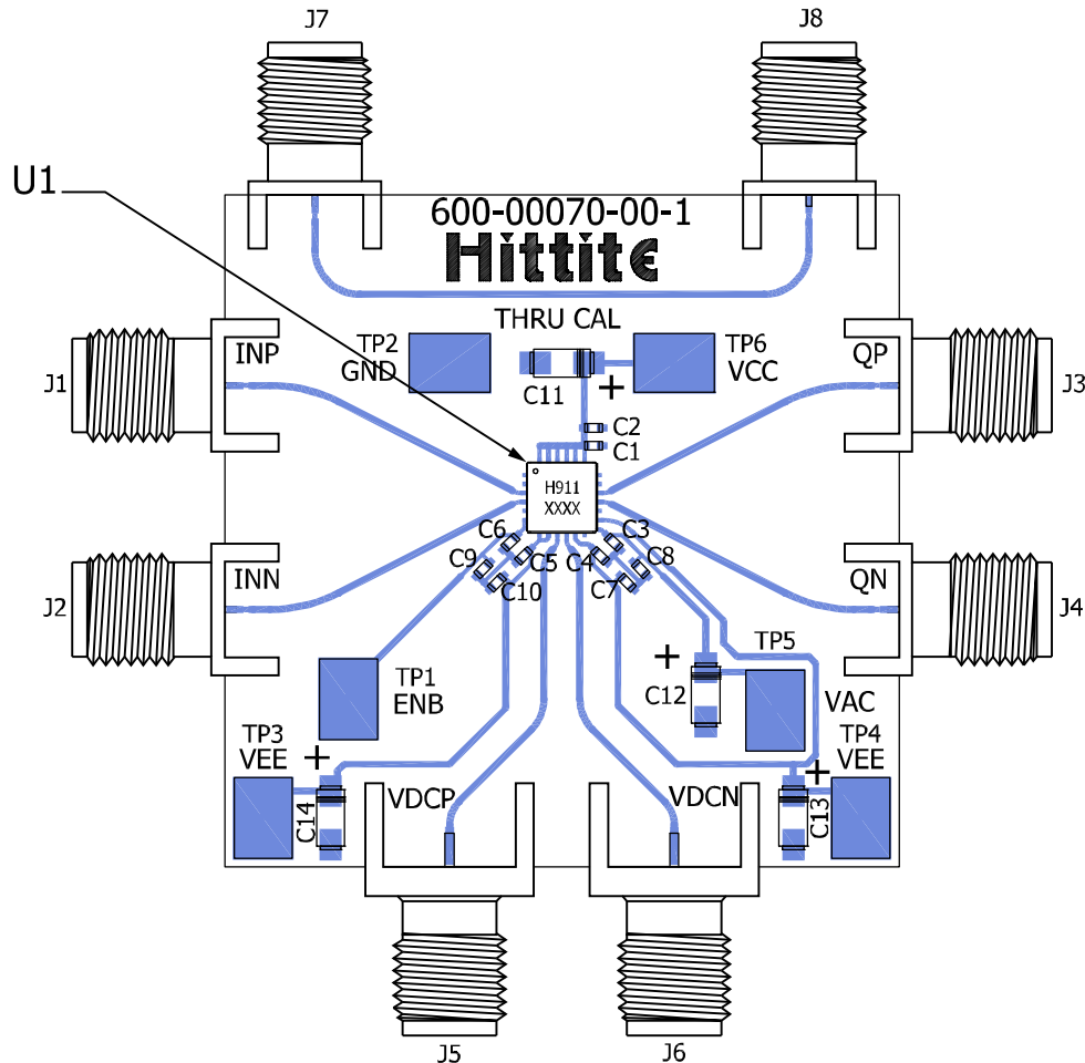
Figure 34. 600-00070-00-1 (EVAL01-HMC911LC4B) Evaluation Board
