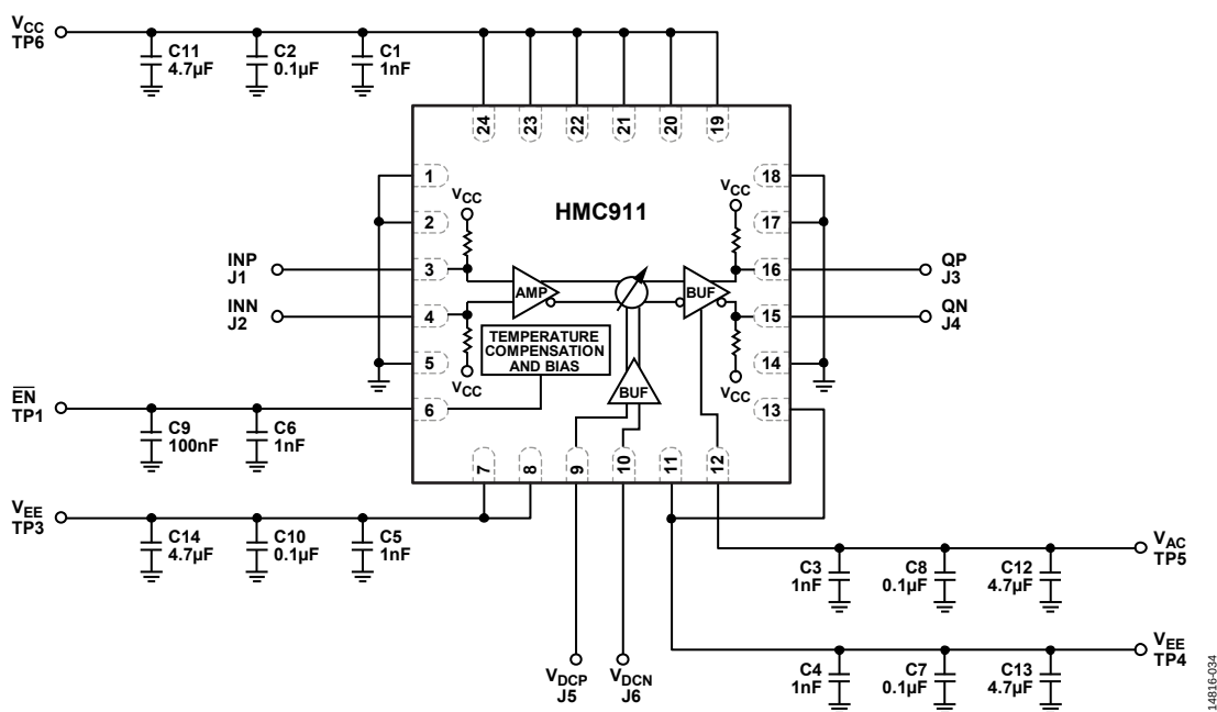
Figure 35. Typical Application Circuit
