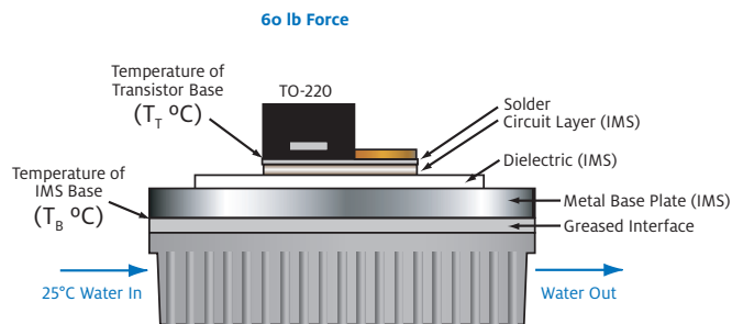
Water-cooled Heatsink
