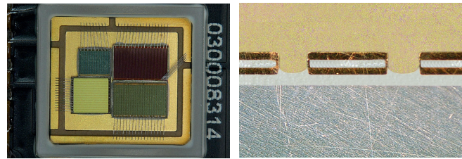
Close-up view of direct die attachment in an LED application. The THERMAL CLAD substrate is used to mount the die or module.
