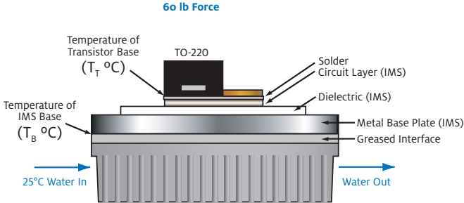
Water-cooled Heatsink
