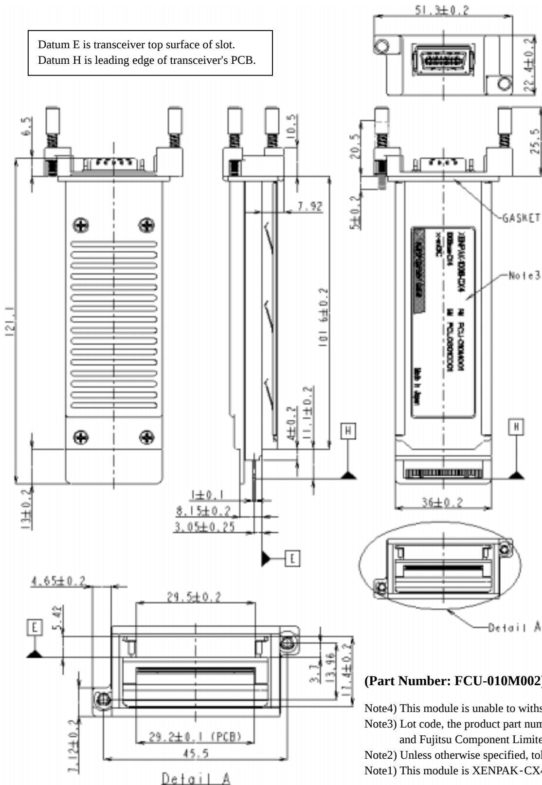
Figure 8: Mechanical Design
