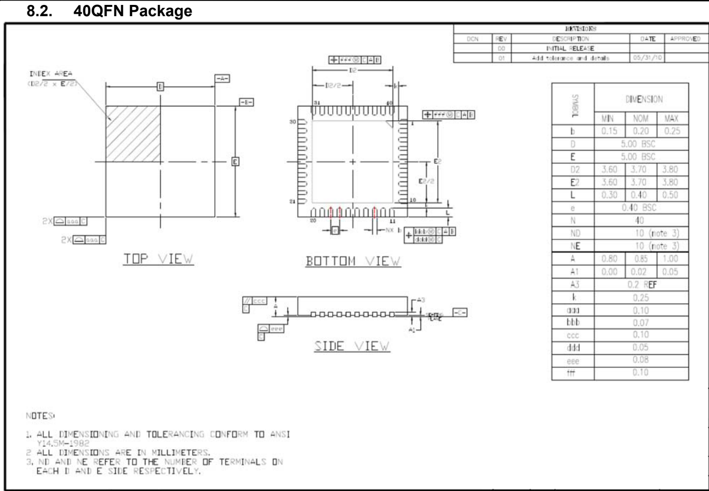
Figure 15. 40QFN Package Drawing
