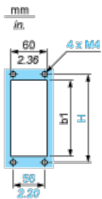
Panel cut-out
