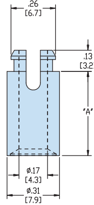
TWO PRONG SNAP LOCK / #8 SELF-TAPPING SCREW
