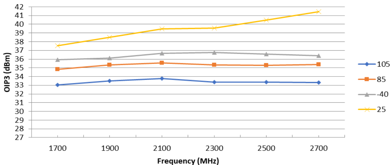
GRF2071 OIP3 vs. Frequency vs. Temperature
