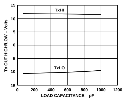
Figure 11. Transmitter Output Voltage High/Low vs. Load Capacitance
