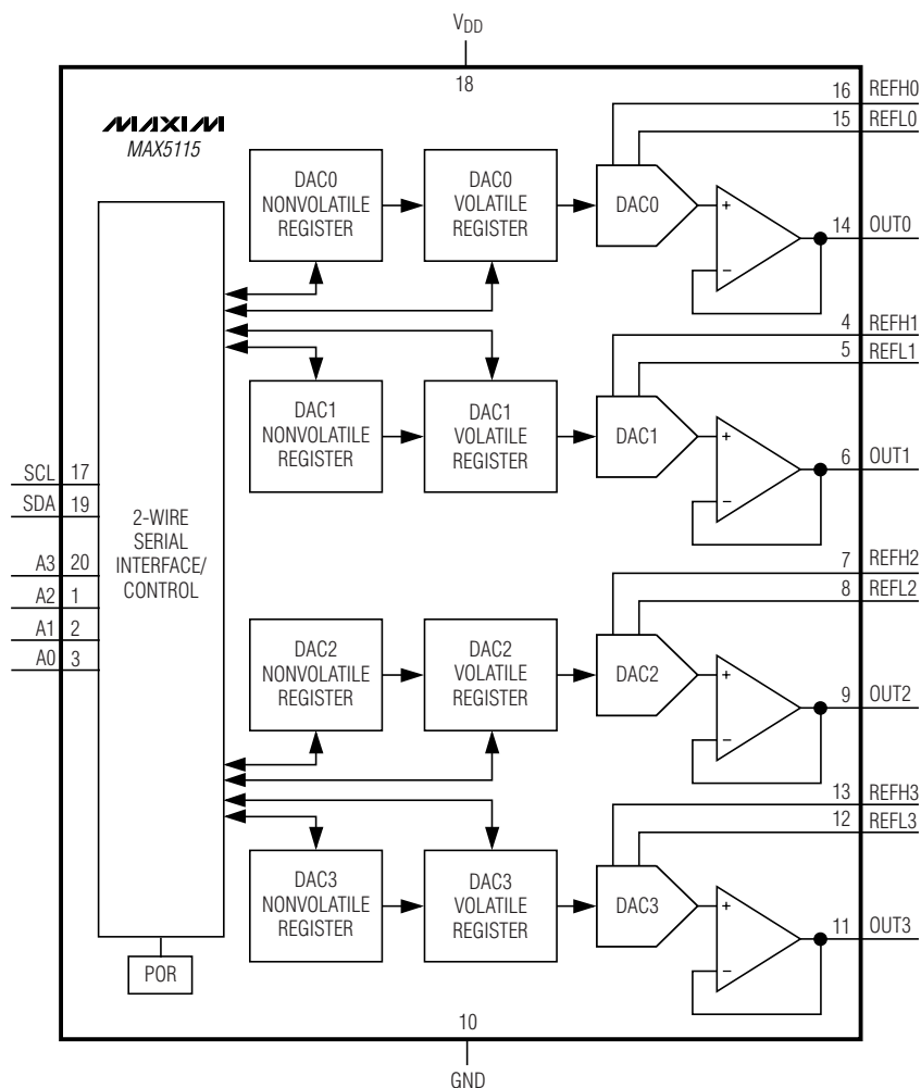
Figure 1. MAX5115 Functional Diagram
