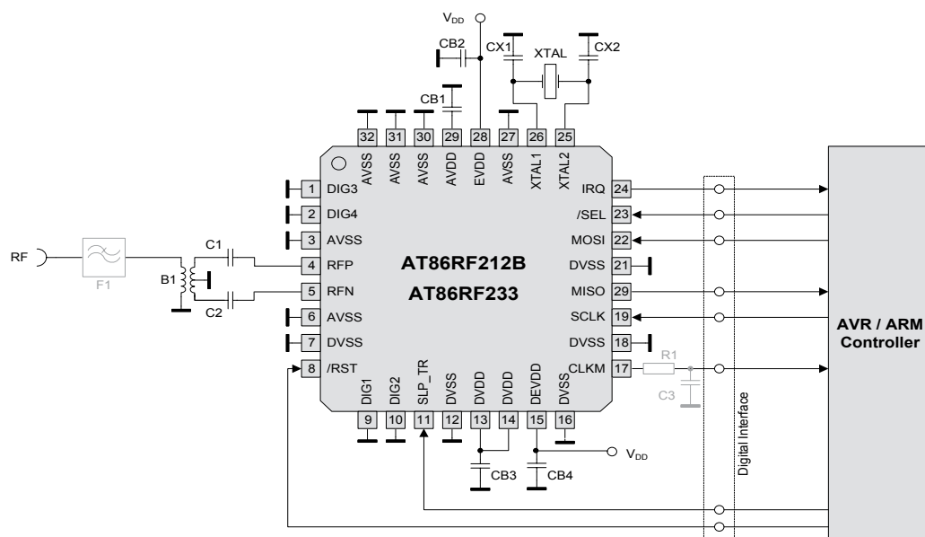
Figure 13. Wireless Tranceiver Application Diagram
