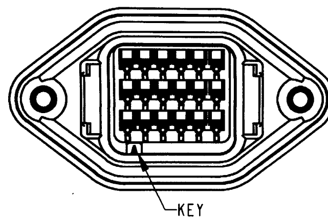
DTV02-18PA KEY ARRANGEMENT -A- COLOR: GREY
