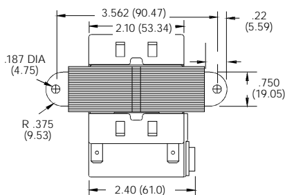
Type BB Same Side Termination
