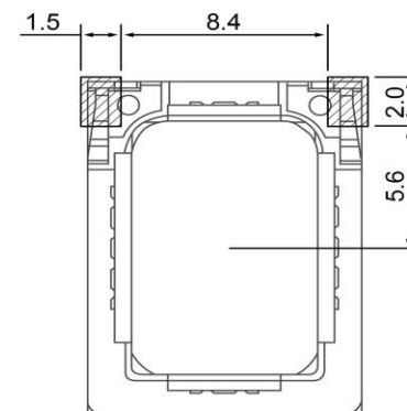
RECOMMENDABLE LAND PATTERN
