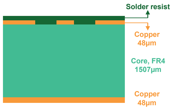
Figure 14. PCB stack-up recommendations
