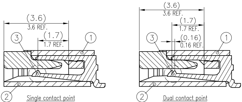
SECTION X-X
