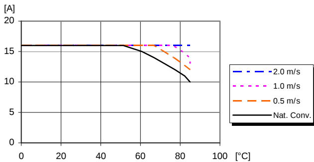
Available load current vs. ambient air temperature and airflow at V_i = 5\text{ V} . See Thermal Consideration section.
