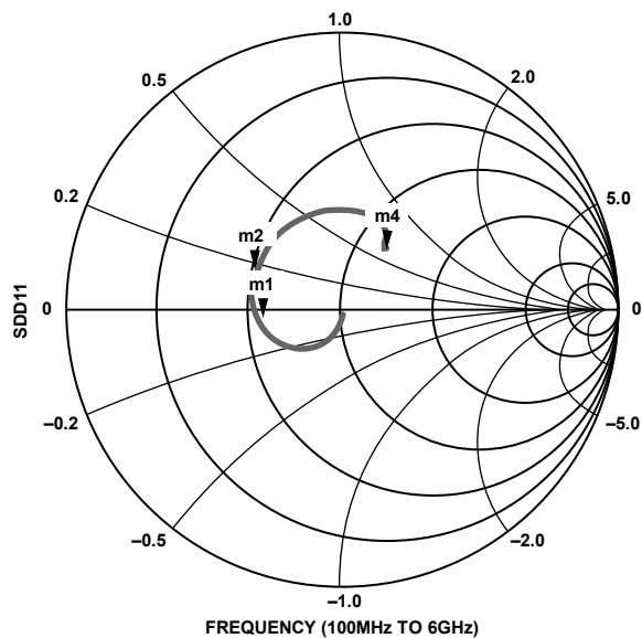
Figure 62. Differential Input Return Loss for the CLK± Inputs
