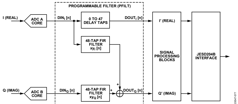
Figure 82. 48-Tap Half Complex Filter Configuration
