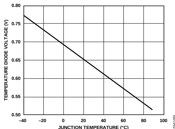
Figure 74. Typical Voltage Response of the 1× Temperature Diode
