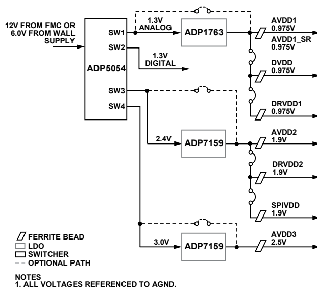
Figure 132. Simplified Power Solution for the AD9208
