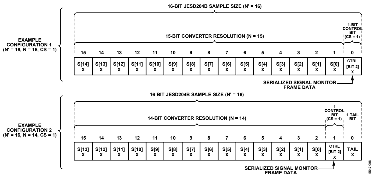
Figure 103. Signal Monitor Control Bit Locations
