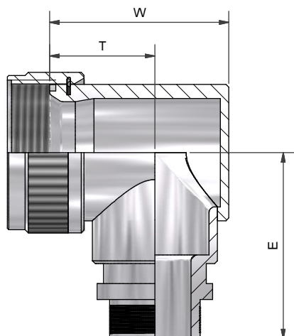
90° BACKSHELL - TYPE 1
