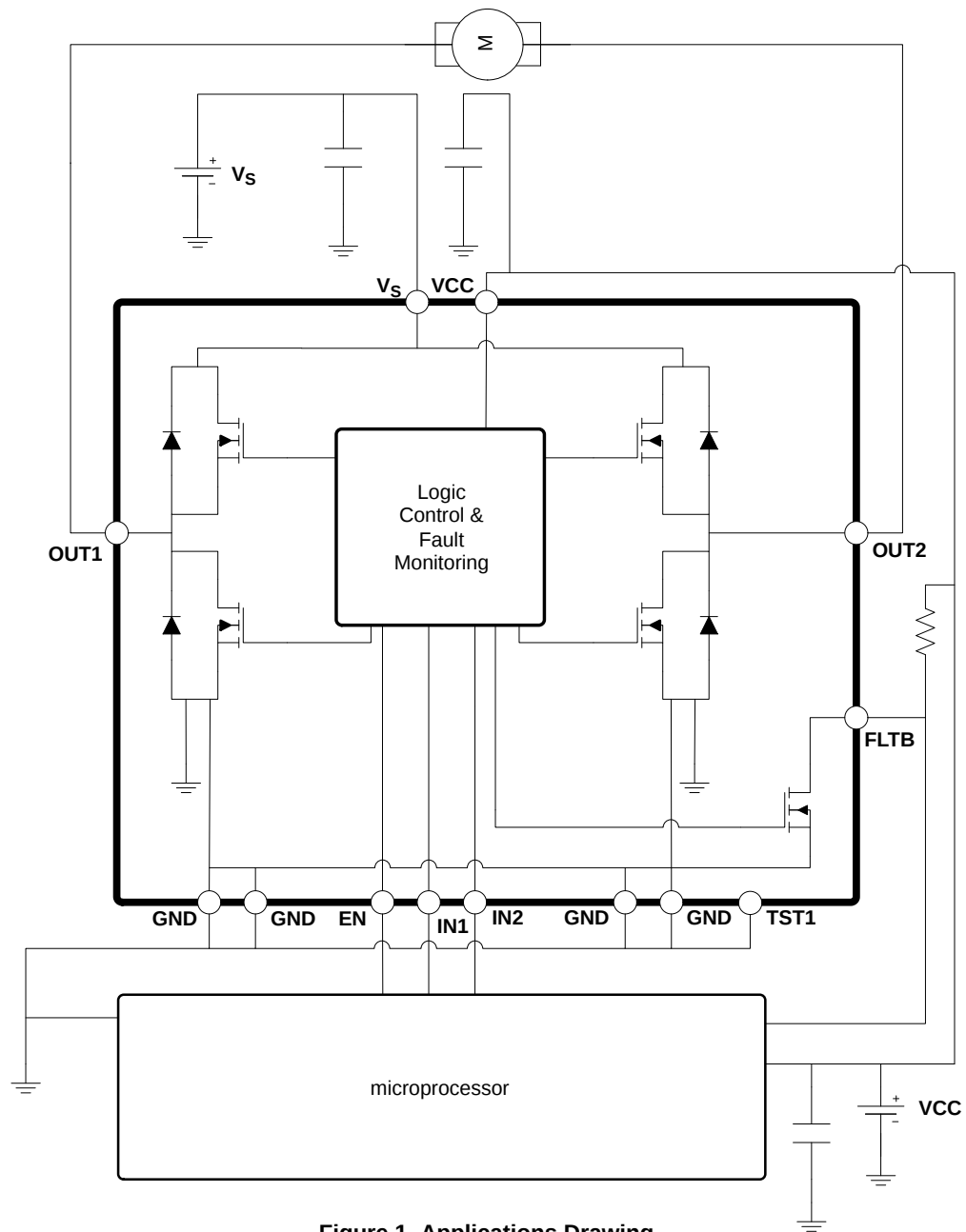
Figure 1. Applications Drawing
