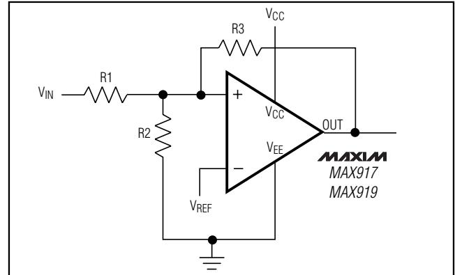
Figure 3. MAX917/MAX919 Additional Hysteresis
