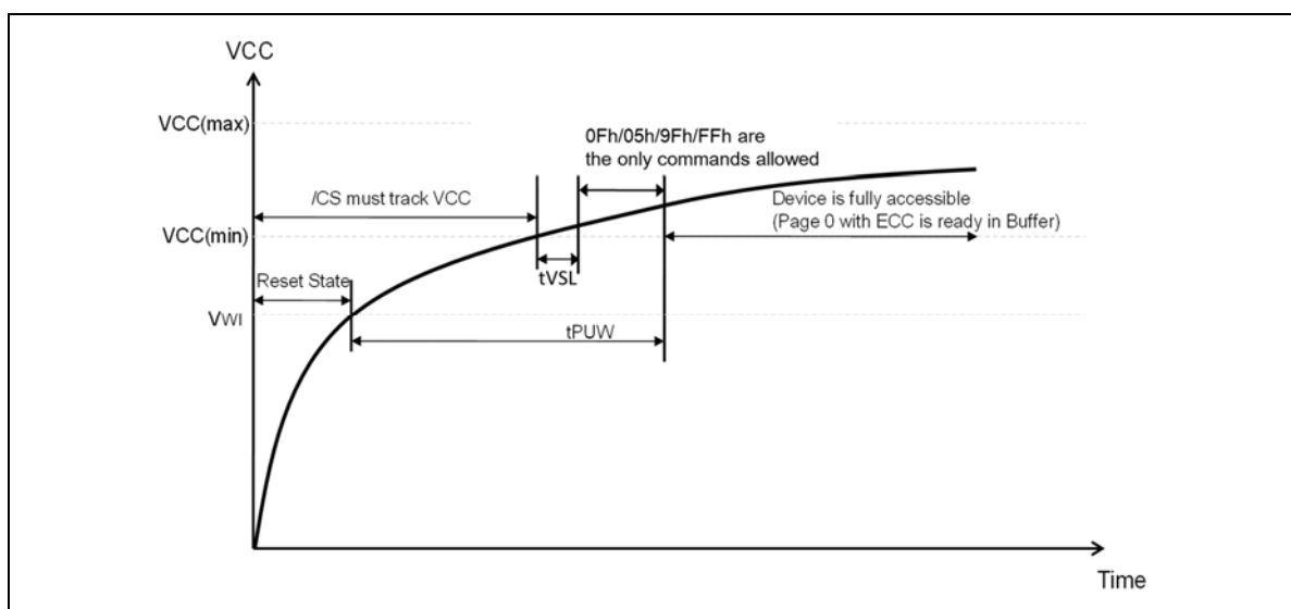
Figure 30a. Power-up Timing and Voltage Levels
