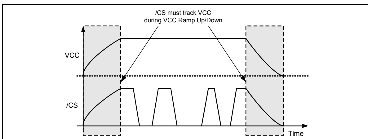
Figure 30b. Power-up, Power-Down Requirement
