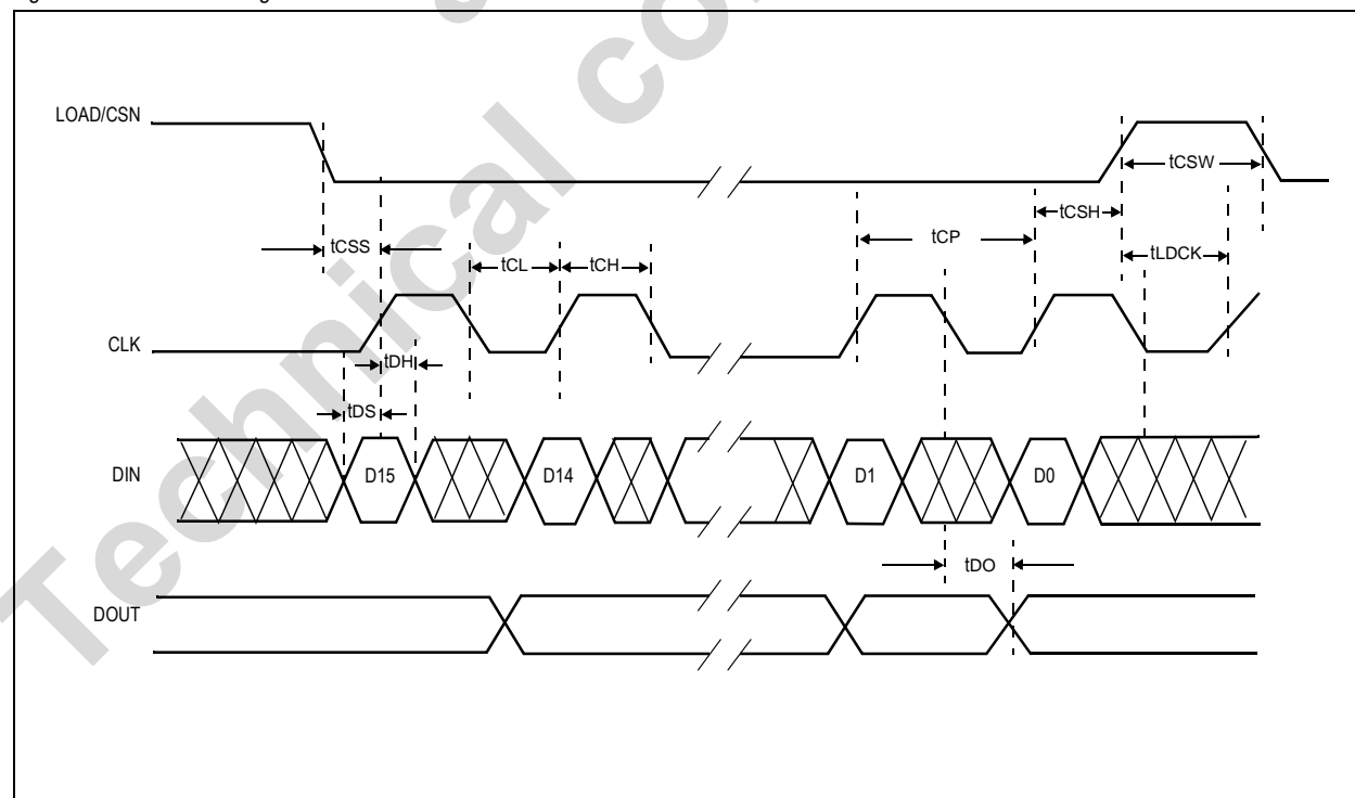
Figure 12. Interface Timing
