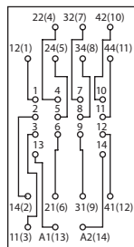
CONNECTION DIAGRAM
