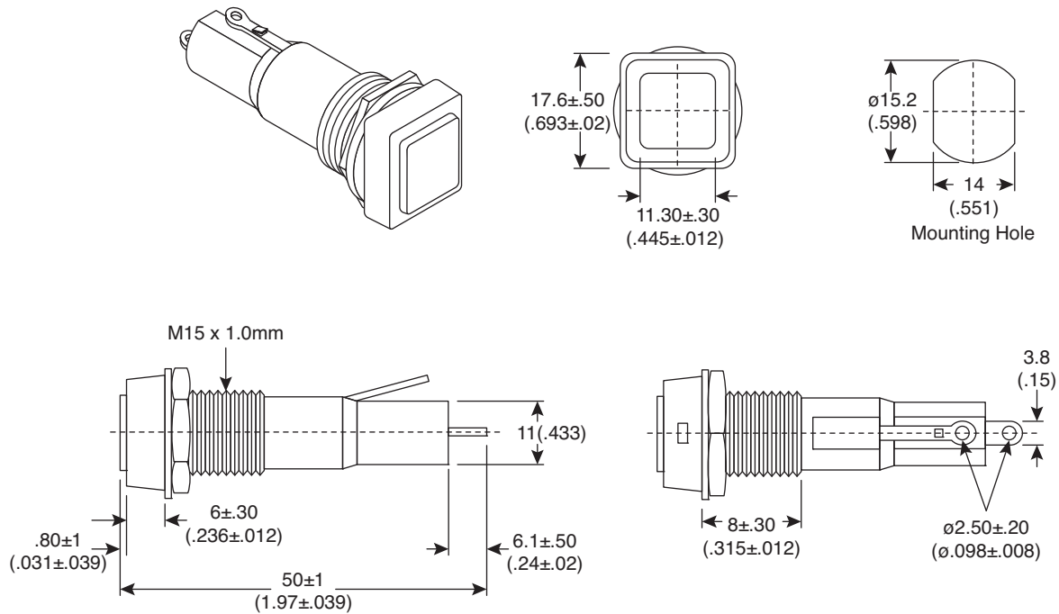
Dimensions: mm (in.)
