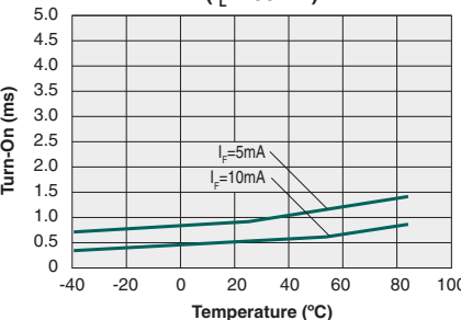
Typical Turn-On vs. Temperature ( I_L=100\text{mA} )
