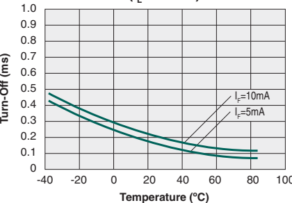
Typical Turn-Off vs. Temperature ( I_L=100\text{mA} )
