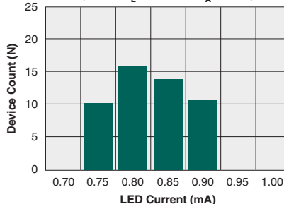
Typical I_F for Switch Dropout (N=50, I_L=100\text{mA} , T_A=25^\circ\text{C} )
