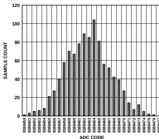
Figure 9. Histogram (Analog Input Buffers Disabled, V_{REF} = 5\text{ V} , Output Data Rate = 10 kSPS)
