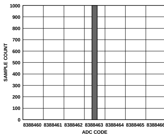
Figure 8. Histogram (Analog Input Buffers Disabled, V_{REF} = 5\text{ V} , Output Data Rate = 5 SPS)
