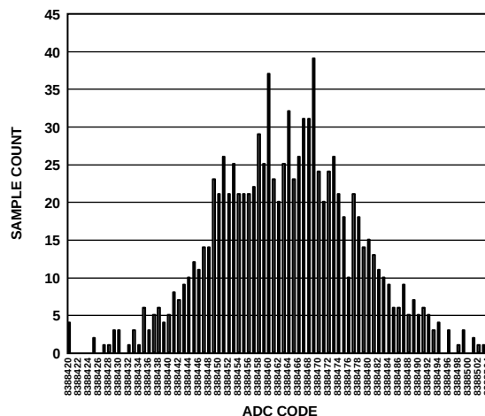
Figure 10. Histogram (Analog Input Buffers Disabled, V_{REF} = 5\text{ V} , Output Data Rate = 250 kSPS)
