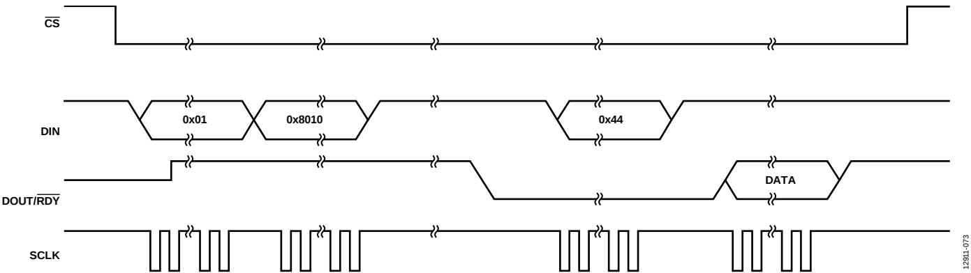
Figure 69. Single Conversion Mode
