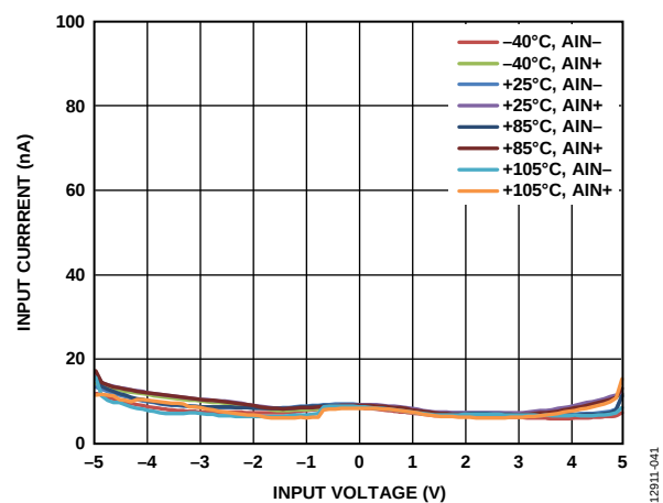
Figure 40. Analog Input Current vs. Input Voltage ( V_{CM} = 2.5\text{ V} )
