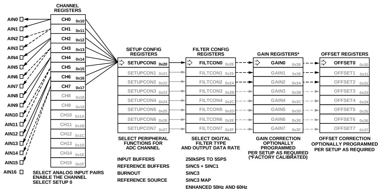
Figure 47. Eight Fully Differential Inputs, All Using a Single Setup (SETUPCON0; FILTERCON0; GAIN0; OFFSET0)
