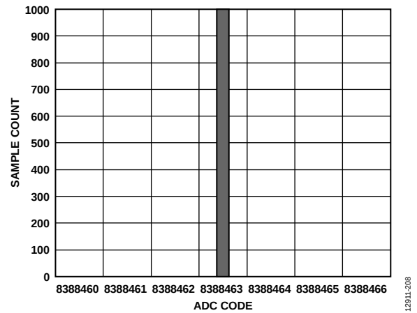
Figure 8. Histogram (Analog Input Buffers Disabled, V_{REF} = 5 V, Output Data Rate = 5 SPS)
