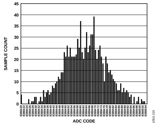
Figure 10. Histogram (Analog Input Buffers Disabled, V_{REF} = 5 V, Output Data Rate = 250 kSPS)
