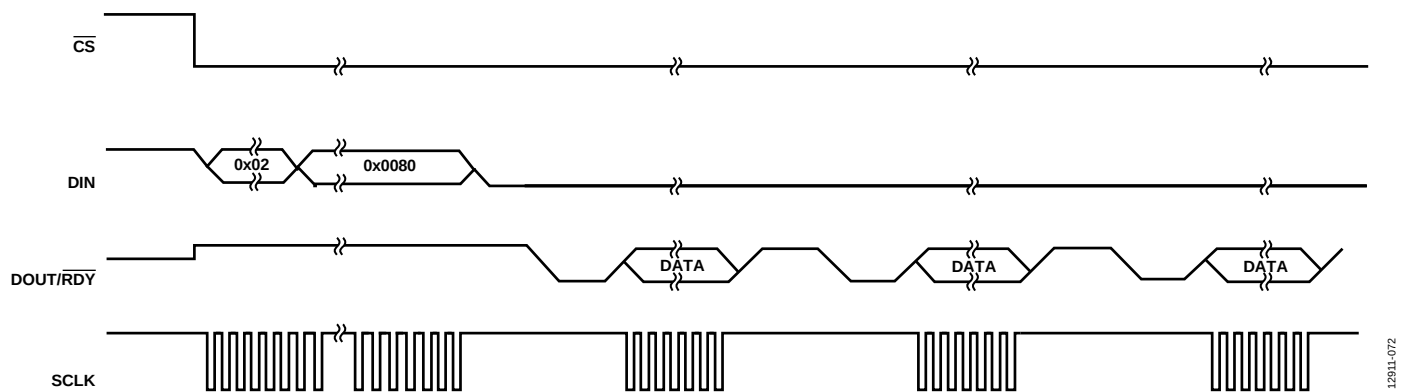
Figure 68. Continuous Read Mode
