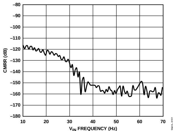
Figure 21. Common-Mode Rejection Ratio (CMRR) vs. V_{IN} Frequency ( V_{IN} = 0.1 V, 10 Hz to 70 Hz, Output Data Rate = 20 SPS, Enhanced Filter)
