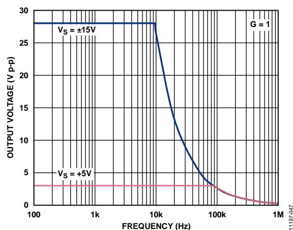
Figure 44. Large Signal Frequency Response
