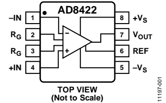
Figure 1. 8-Lead MSOP (RM), 8-Lead SOIC (R)
