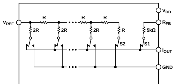
Figure 18. Equivalent R-2R DAC Circuit
