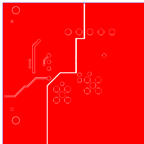
Figure 30. Solder Side Artwork
