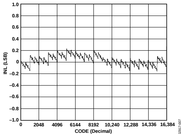
Figure 9. AD5553 INL Error
