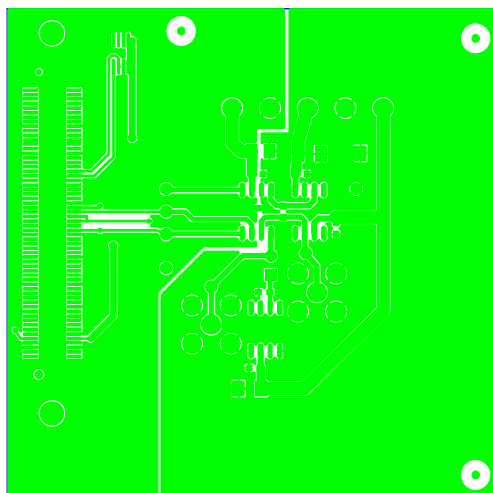
Figure 29. Component Side Artwork
