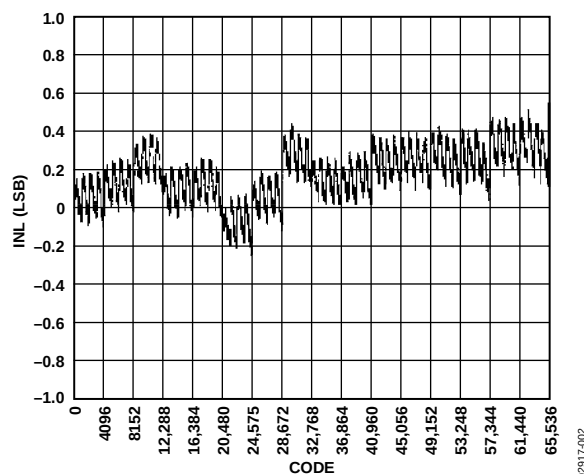
Figure 2. Integral Nonlinearity (INL)
