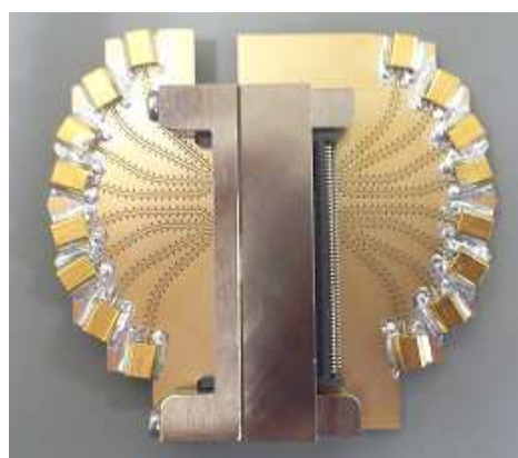
PN:CN:121-PCB ( Measure with GPPO connector )
