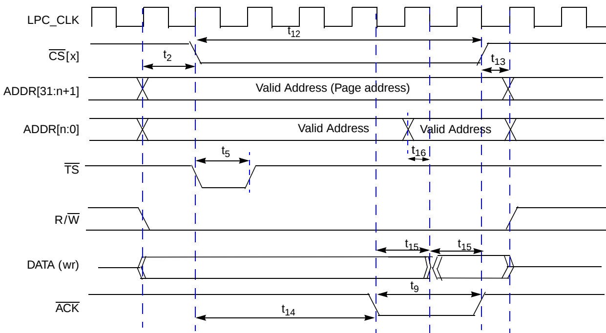
Figure 17. Timing Diagram – Non-MUXed Aynchronous Write Burst
