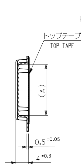
SECT:X-X
