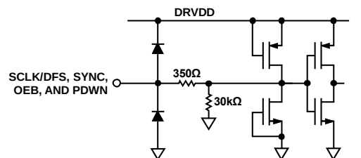
Figure 38. Equivalent SCLK/DFS, SYNC, OEB, and PDWN Input Circuit
