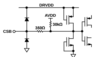
Figure 40. Equivalent CSB Input Circuit
