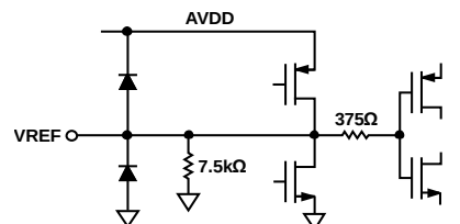
Figure 41. Equivalent VREF Circuit
