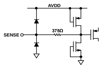
Figure 39. Equivalent SENSE Circuit
