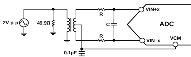
Figure 45. Differential Transformer-Coupled Configuration
