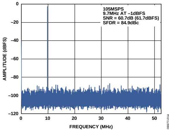
Figure 23. Single-Tone FFT with f_{IN} = 9.7 MHz
