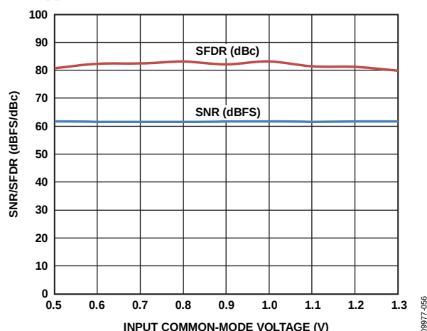
Figure 43. SNR/SFDR vs. Input Common-Mode Voltage, f_{IN} = 70 \text{ MHz} , f_s = 125 \text{ MSPS}
