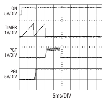
Power-Up Waveforms
