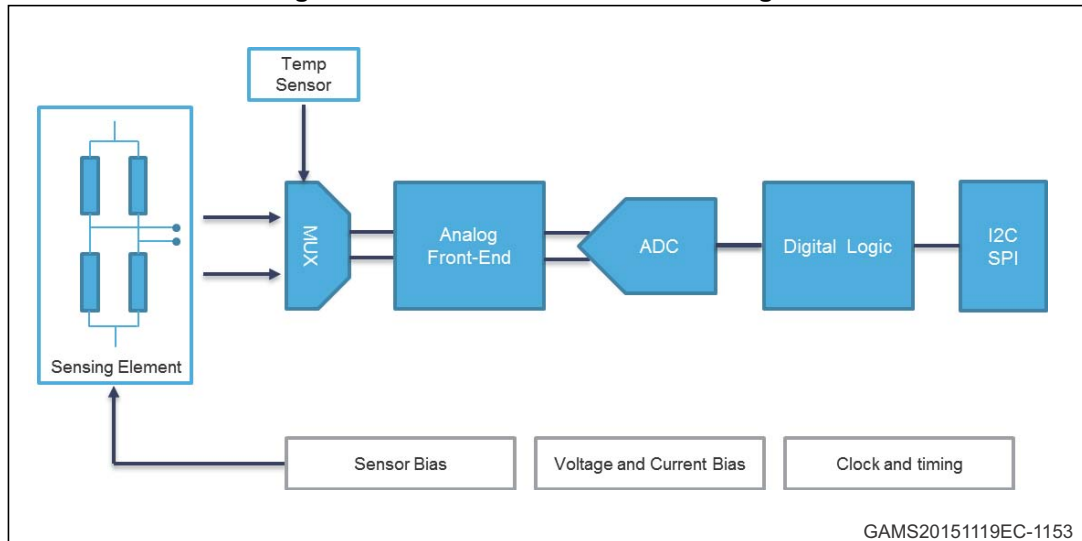
Figure 2. Digital logic
