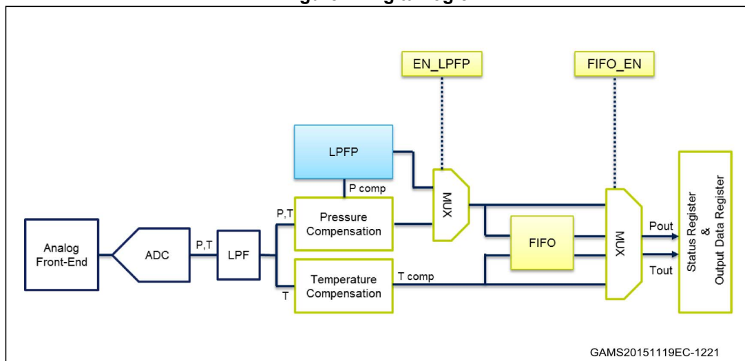
Figure 2. Digital logic
