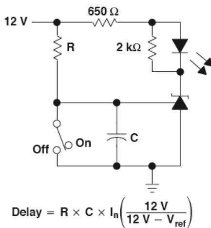
Figure 14: Delay Timer
