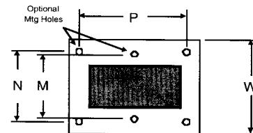
Mounting Hole Drawing
