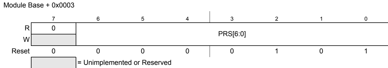
Figure 10-7. ADC Timing Register (ADCTIM))
