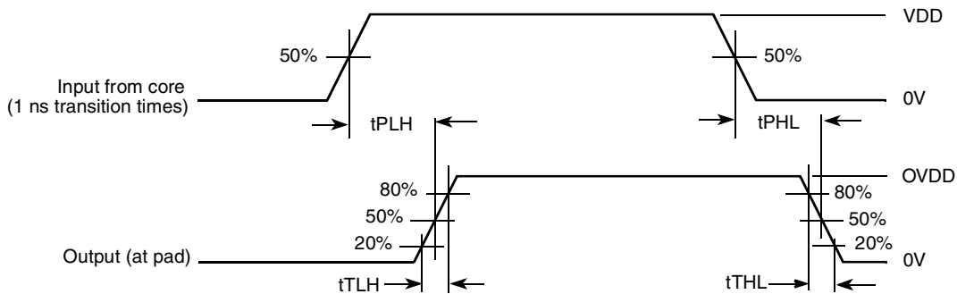
Figure 5. Output Pad Propagation and Transition Time Waveform
